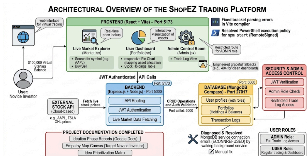
Figure 1: MERN Stack Architecture and Data Flow for Shoez Virtual Trading Simulator
